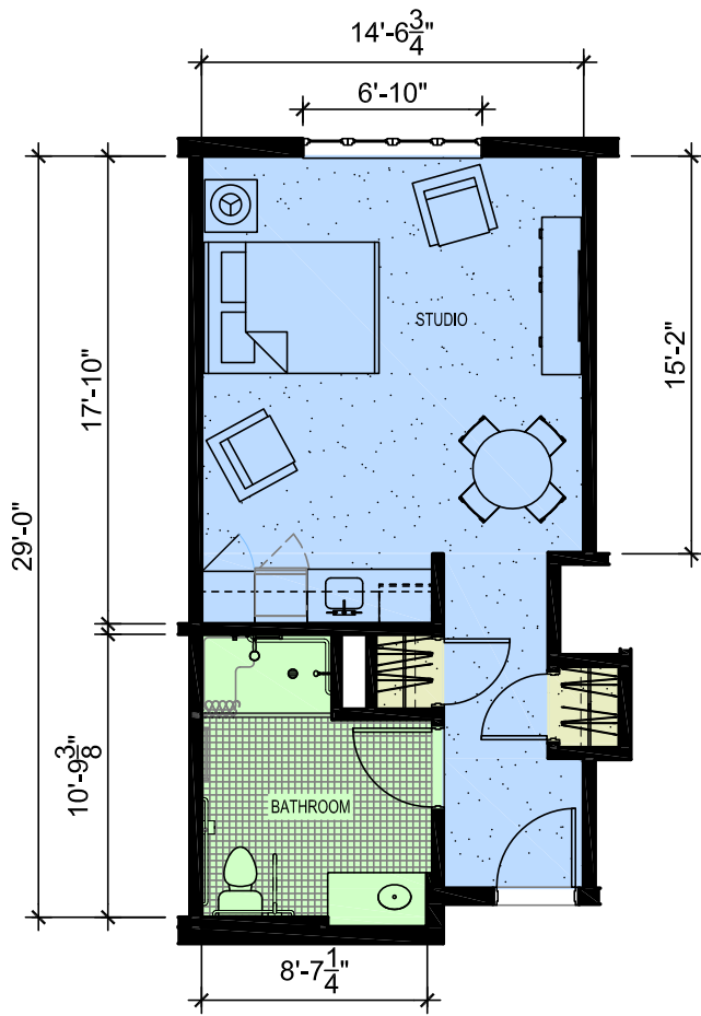
STUDIO APARTMENT (422 S.F.)
